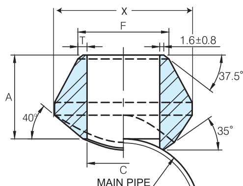
STRAIGHT WAY
