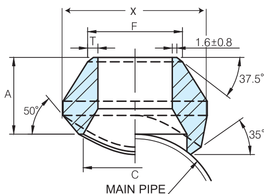
REDUCING WAY
